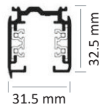
Ceiling Track
