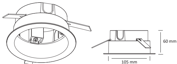
XTSA 71 : Building-in box for GA 70
