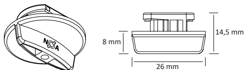
GA 69 : 3-circuits track adaptor. Payload 49N
