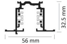
Recessed Track
