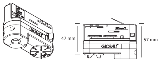
XTSA 71 : Building-in box for GA 70
