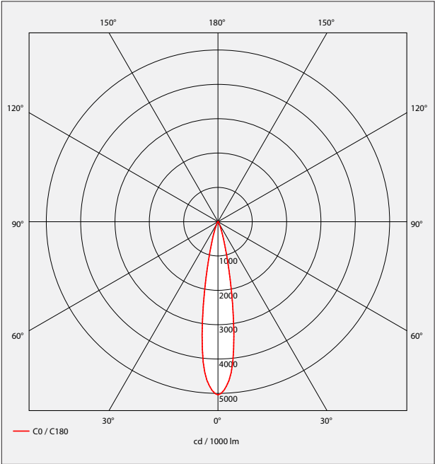
Beams 20° LOR 78,5%
