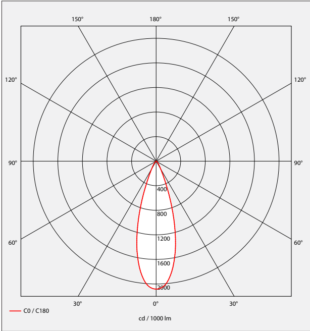
Beams 33° LOR 75%
