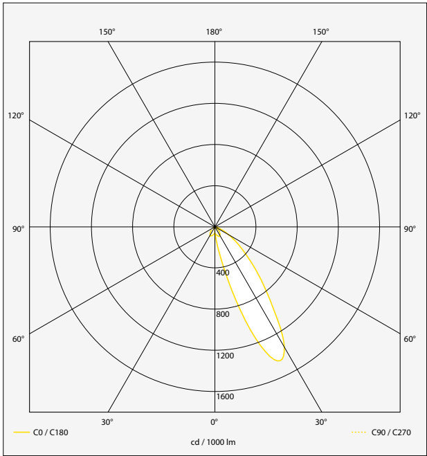
Asymmetrical: LOR 92 %
