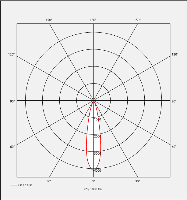
Beams 20° LOR 73,7%
