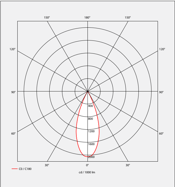
Beams 40° LOR 78%
