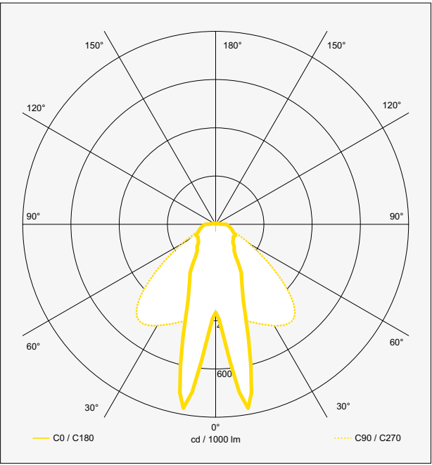
Intensive LOR: 91 %
