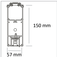
Integration into a profile SE 3516
