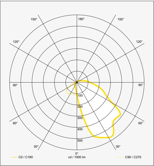
Asymmetrical LOR: 91 %
