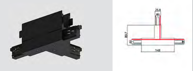
T connector
