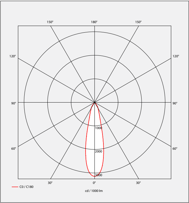
Beams 30° LOR 88,8%
