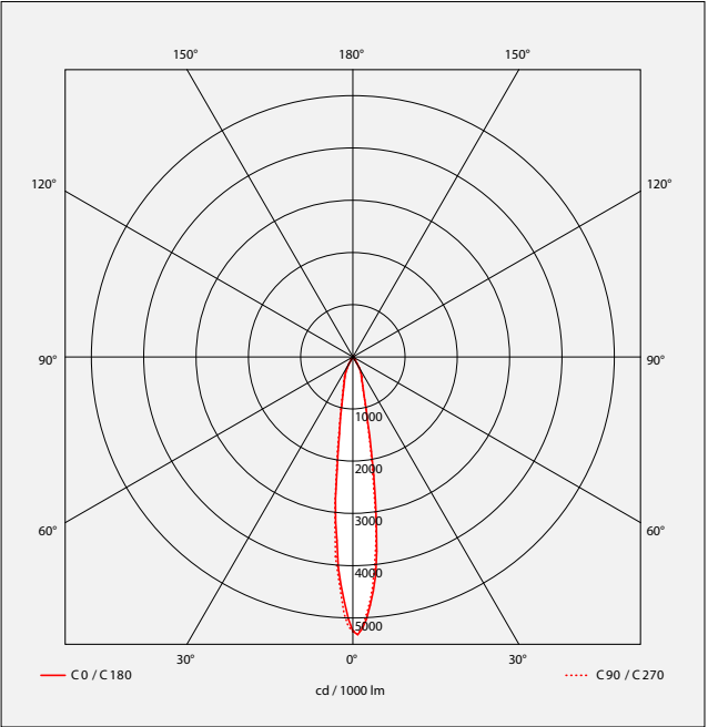
Beams 15°
