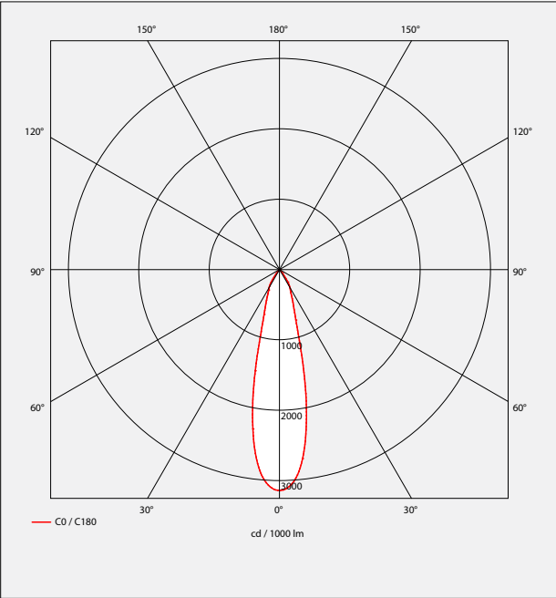
Beams 30° LOR 78,8%
