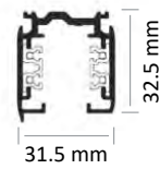
Ceiling Track
