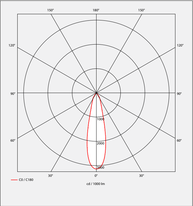
Beams 30° LOR 78,8%
