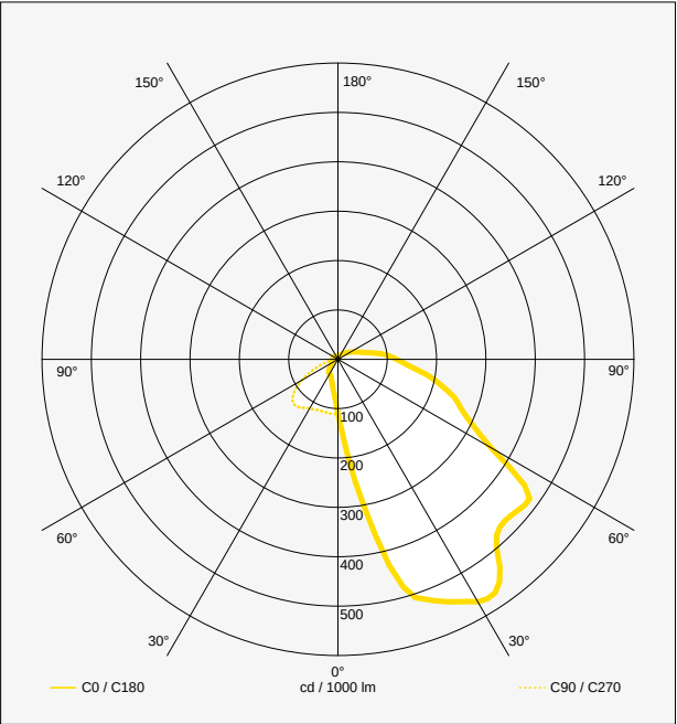
Asymmetrical LOR: 91 %
