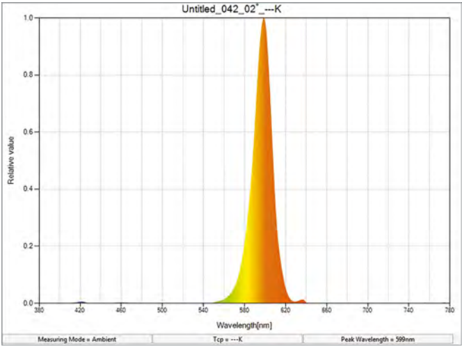
Spectral distribution
