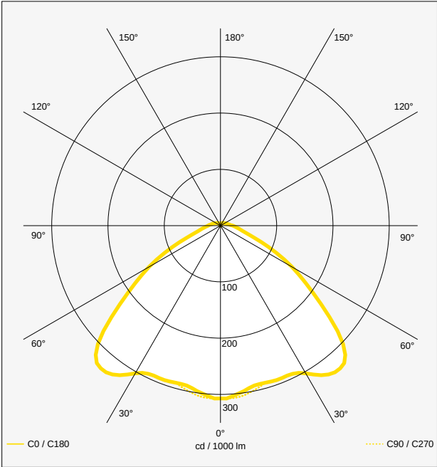
Symmetrical LOR: 95 %
