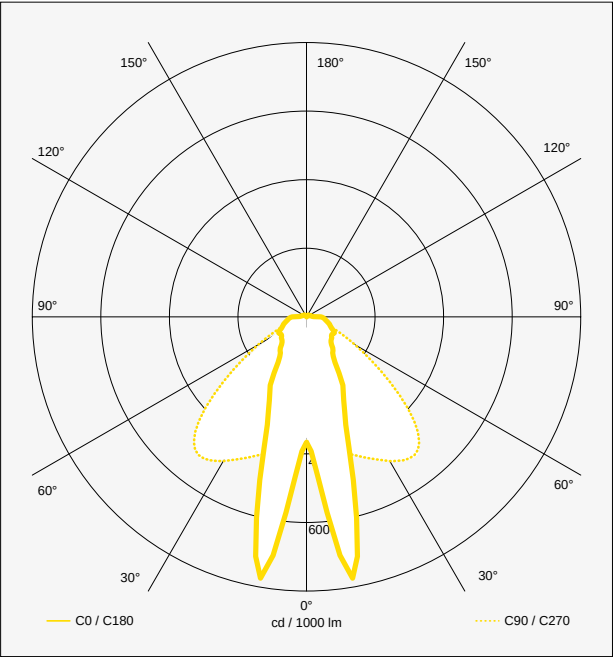
Intensive LOR: 91 %
