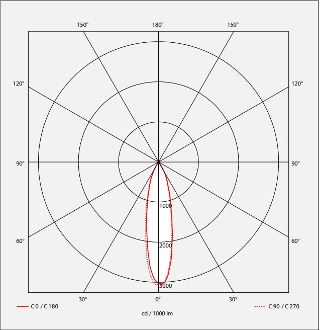
Beams 24°
