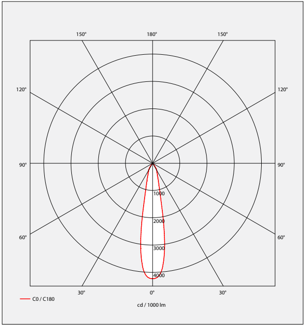
Beams 20° LOR 90,8%
