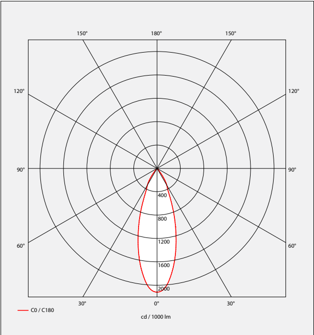
Beams 40° LOR 88,4%
