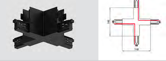
X connector
