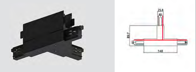
T connector
