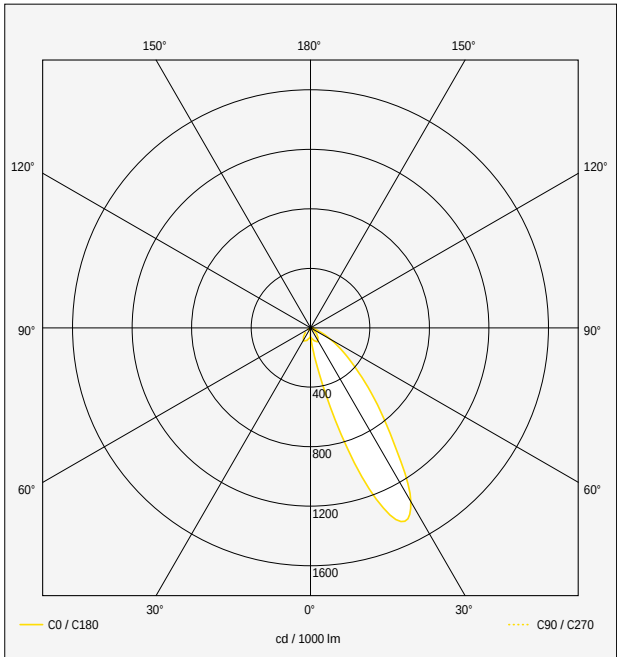
Asymmetrical: LOR 92 %
