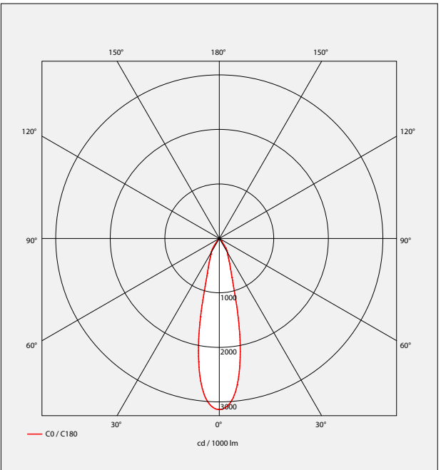
Beams 30° LOR 88,8%
