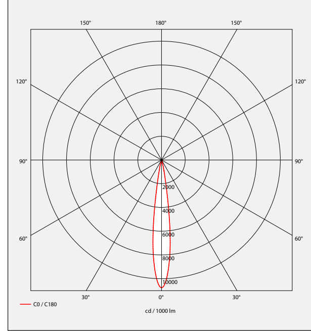
Beams 35° LOR 74,4%
