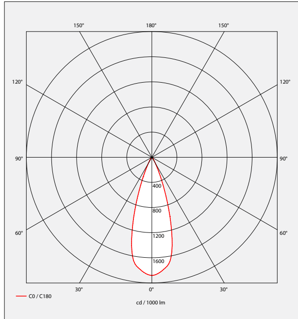
Beams 35° LOR 68,3%
