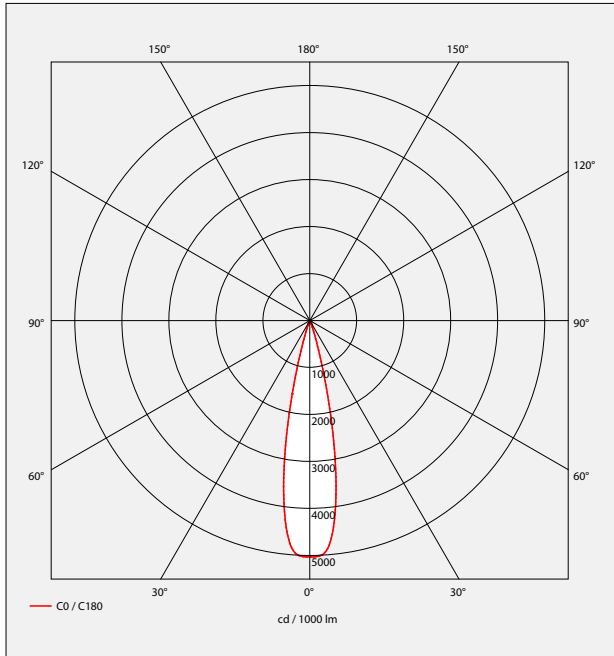
Beams 20° LOR 79.4%
