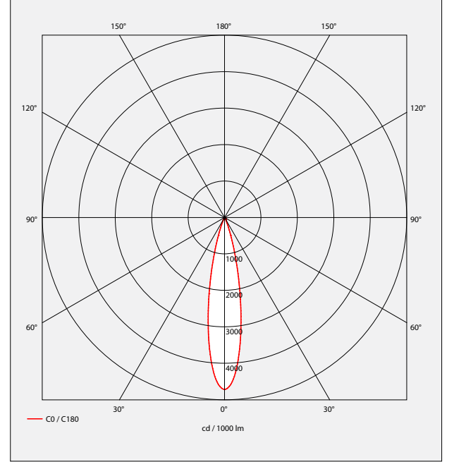
Beams 20° LOR 81,3%
